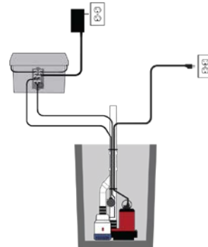
Recommended Installation
